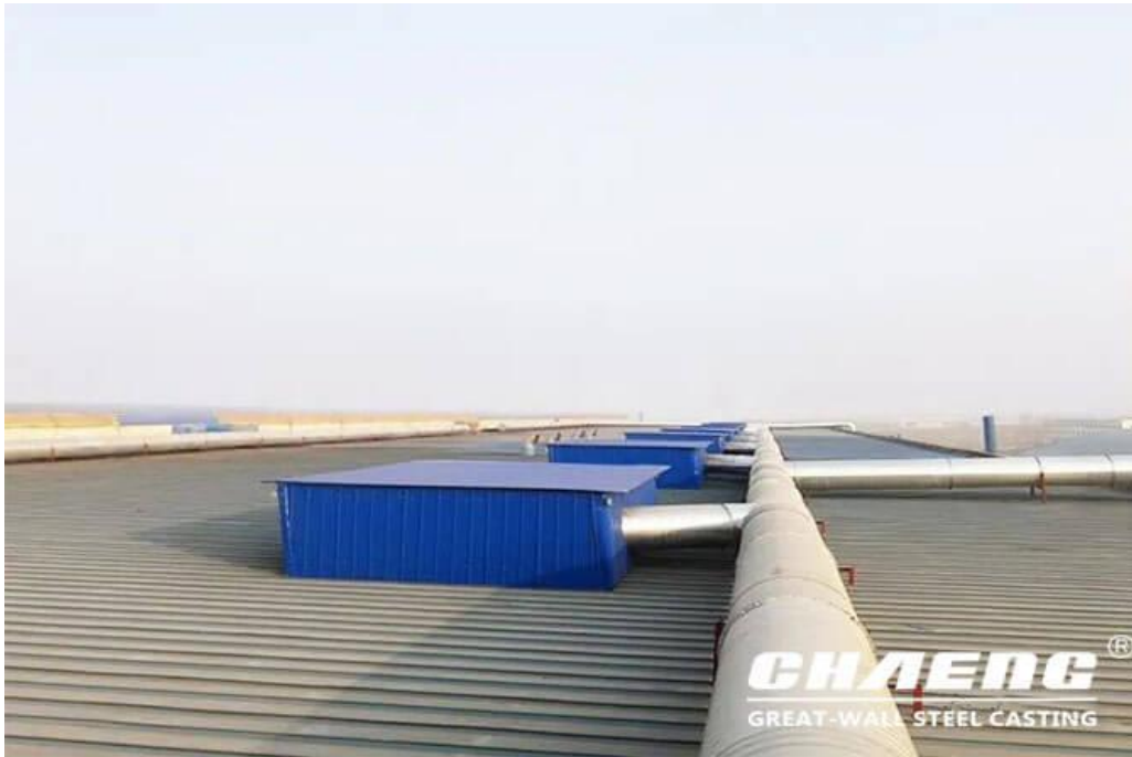
Secondary dust collection pipe of workshop top draft hood
